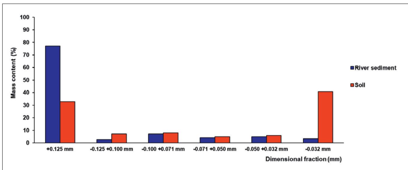
Figure 7. Comparative histogram of mass content of the various dimensional grain fractions
