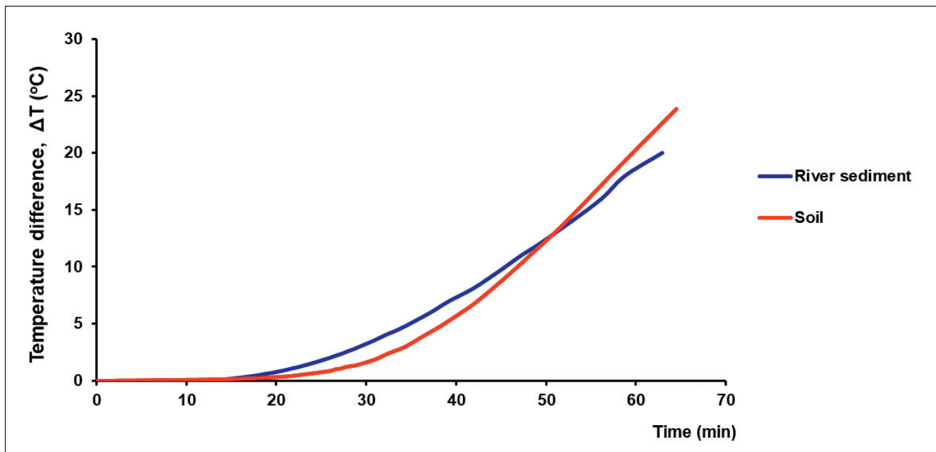
Figure 8. Heat transfer at dry state
