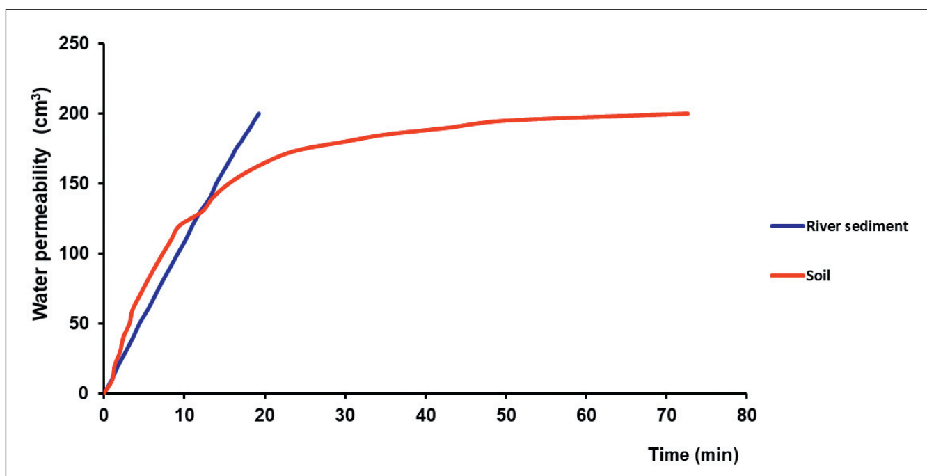
Figure 12. Water permeability
