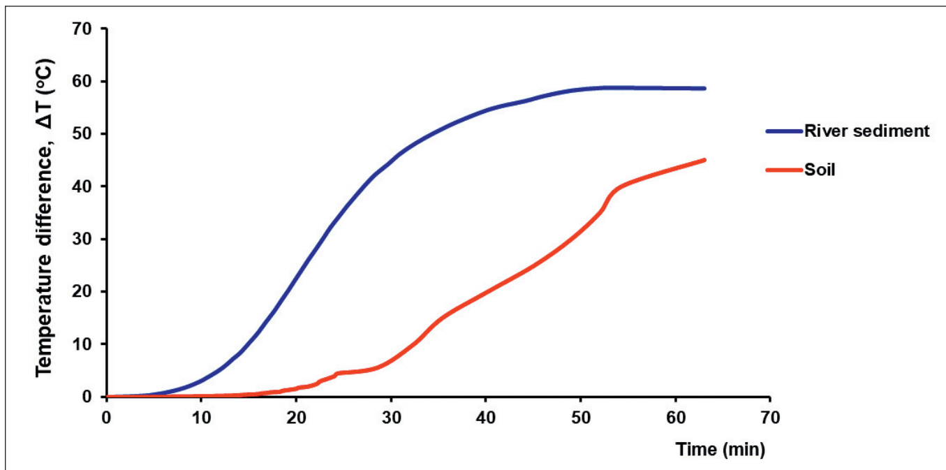
Figure 9. Heat transfer at state of 10 % moisture
